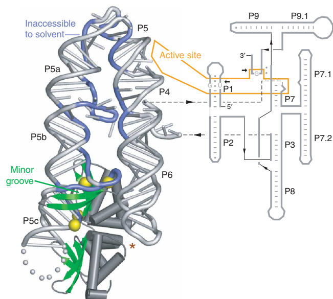
Figure 8 Maturase-facilitated folding of the bI3 intron RNA via action at a distance. The bI3 maturase recognizes a distal structure in a peripheral domain and lies at least 50 Å from the group I intron active site (orange). Green, the maturase \beta -strands; dark gray, the remainder of the protein; light blue, regions protected from solvent-based hydroxyl radical cleavage upon maturase binding; yellow spheres, sulfate groups visualized crystallographically; brown asterisk, a potential auxiliary RNA-protein interaction site.
